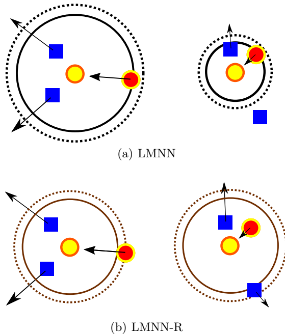
Fig. 2. Illustration contrasting our proposed approach with [9]. Note that the point configurations for a) and b) are the same. For a given training point (yellow), the target neighbor (red) is pulled closer, while the impostors (blue) are pushed away. a) To determine the impostors, the LMNN cost function uses a variable distance from the training point depending on the proximity of the target neighbors; b) LMNN-R on the other hand, forces the impostors out of a universal distance from the training point, while simultaneously attracting target neighbors.
